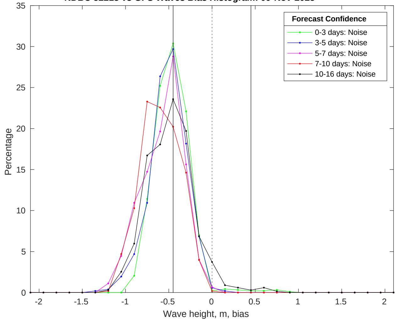
NDBC 52213 vs GFS Waves Bias Histogram: 09-Nov-2025
