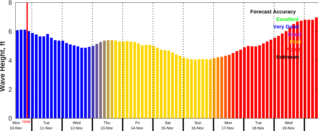
CMEMS Wave Forecast for NDBC 52213 from 09-Nov-2025 11:00:00 to 19-Nov-2025 11:00:00
