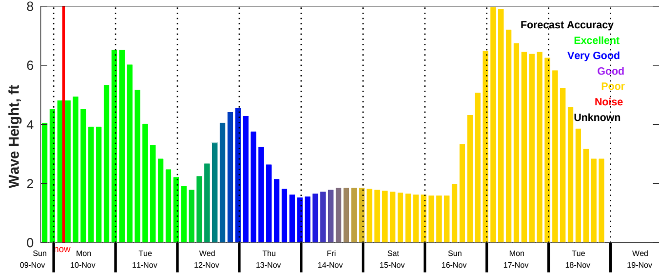
CMEMS Wave Forecast for NDBC 41004 from 09-Nov-2025 19:00:00 to 19-Nov-2025 19:00:00
