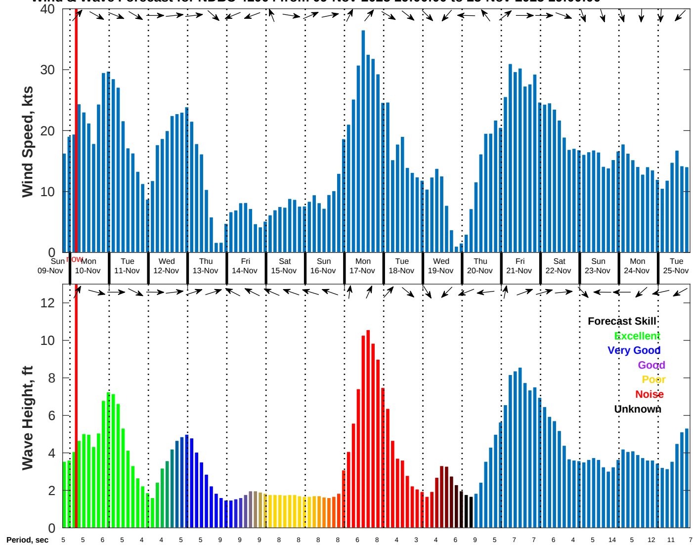
Wind & Wave Forecast for NDBC 41004 from 09-Nov-2025 19:00:00 to 25-Nov-2025 19:00:00
