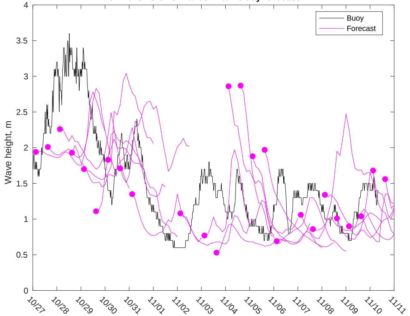
NDBC 41013 vs GFS Waves: 7 to 10 day forecast
