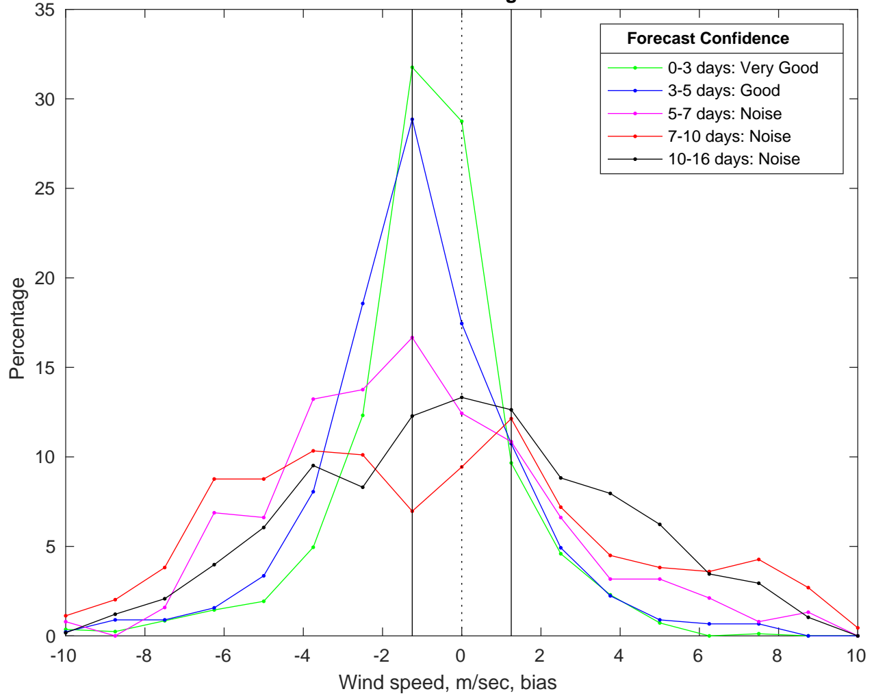
NDBC 41013 vs GFS Winds Bias Histogram: 10-Nov-2025
