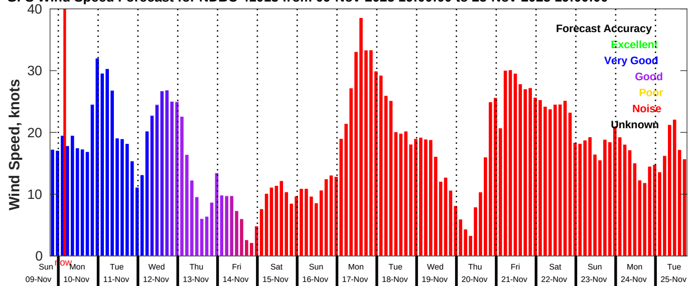
GFS Wind Speed Forecast for NDBC 41013 from 09-Nov-2025 19:00:00 to 25-Nov-2025 19:00:00
