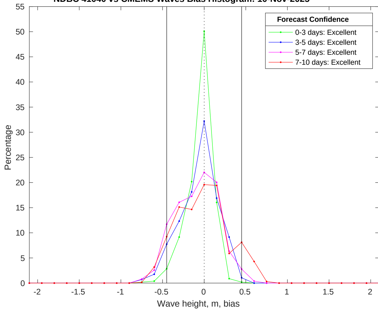
NDBC 41040 vs CMEMS Waves Bias Histogram: 10-Nov-2025
