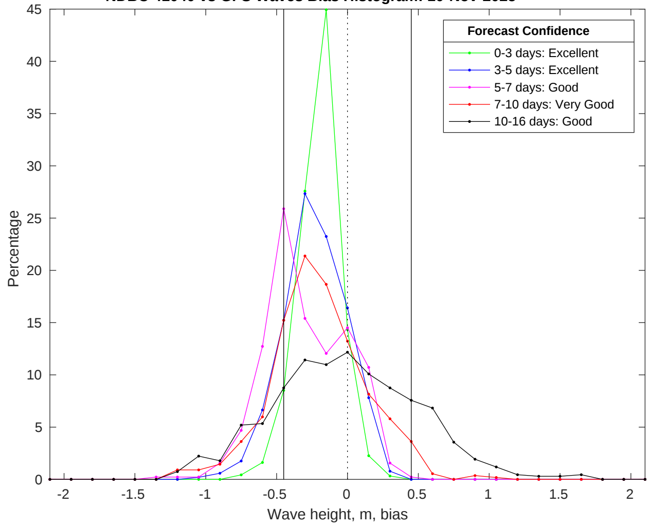
NDBC 41040 vs GFS Waves Bias Histogram: 10-Nov-2025
