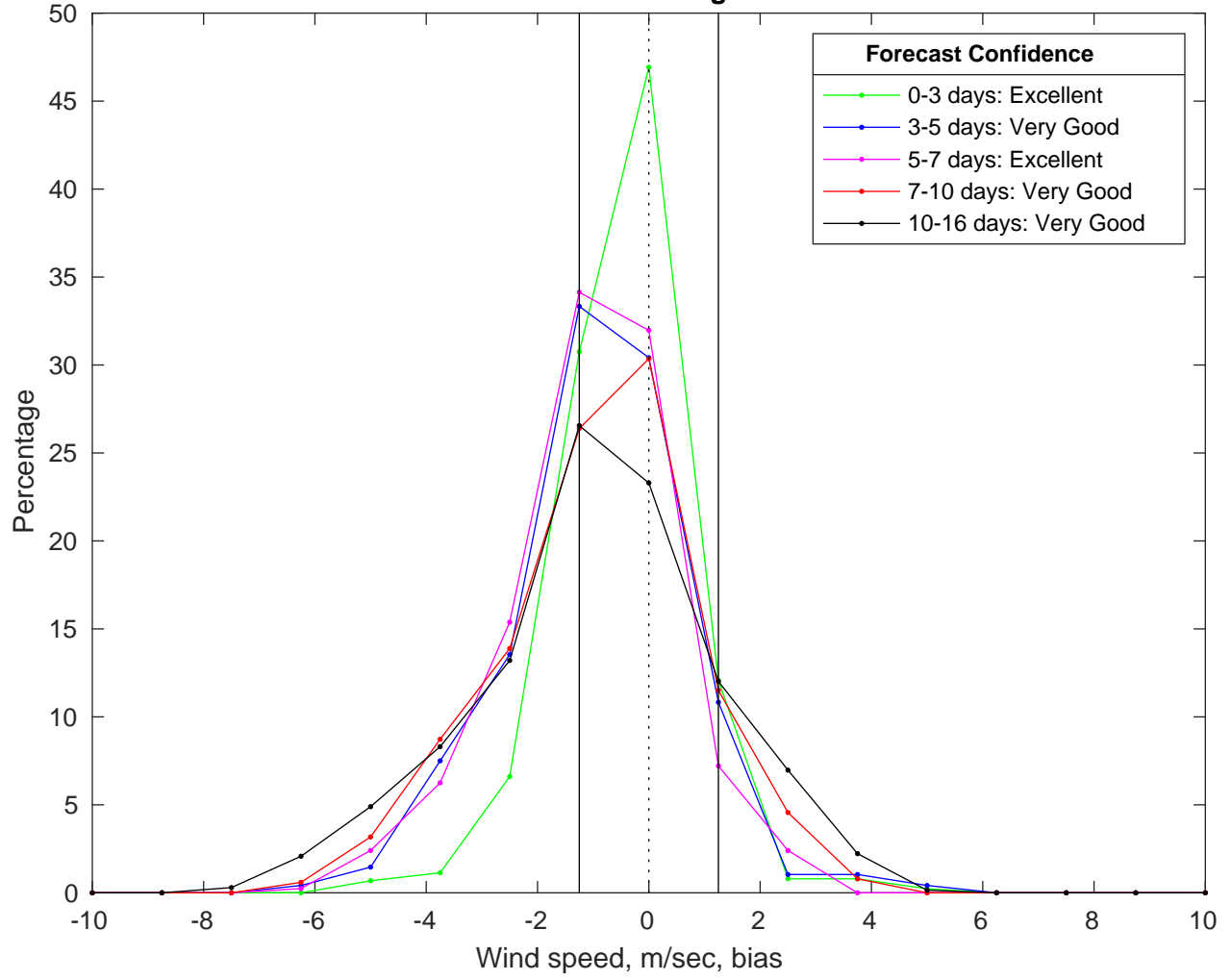
NDBC 41040 vs GFS Winds Bias Histogram: 10-Nov-2025
