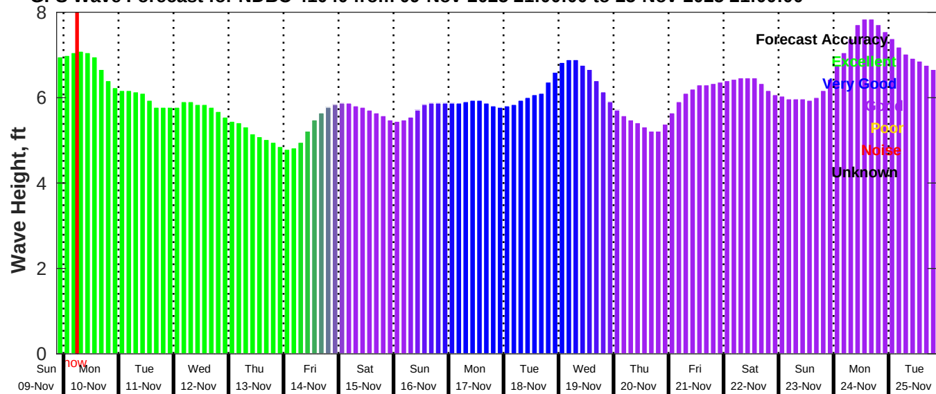
GFS Wave Forecast for NDBC 41040 from 09-Nov-2025 21:00:00 to 25-Nov-2025 21:00:00
