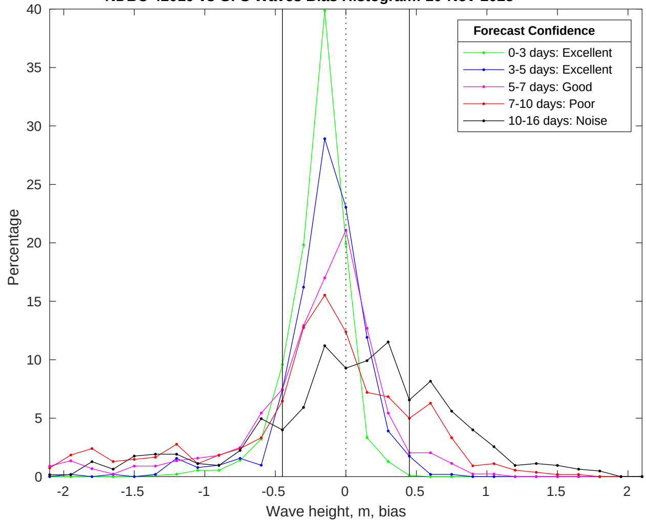
NDBC 42019 vs GFS Waves Bias Histogram: 10-Nov-2025
