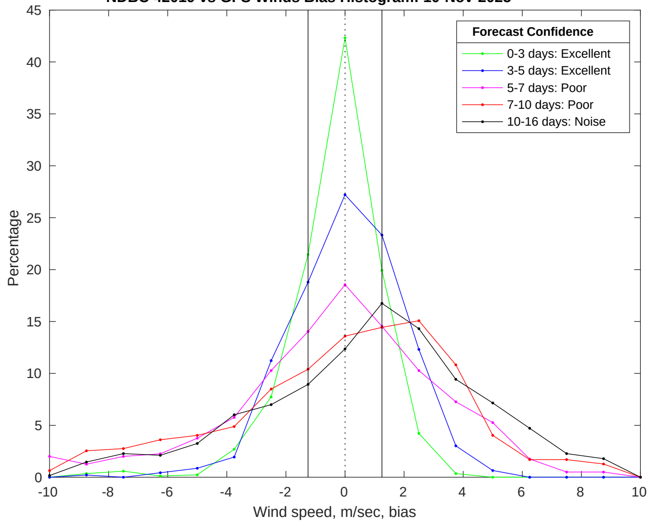
NDBC 42019 vs GFS Winds Bias Histogram: 10-Nov-2025
