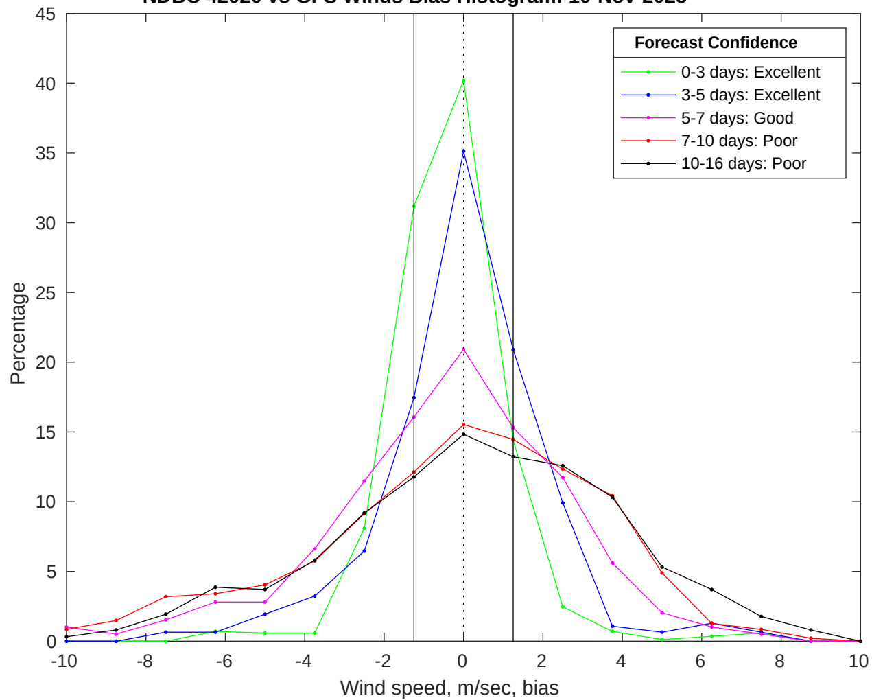
NDBC 42020 vs GFS Winds Bias Histogram: 10-Nov-2025
