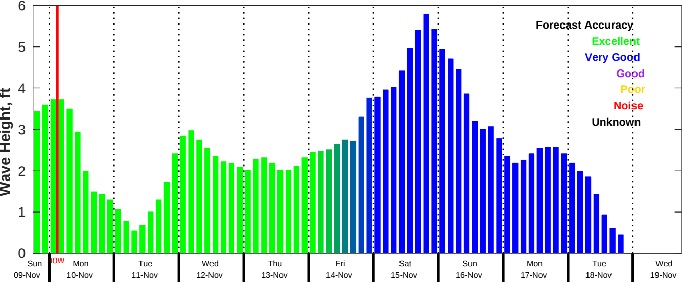
CMEMS Wave Forecast for NDBC 42035 from 09-Nov-2025 18:00:00 to 19-Nov-2025 18:00:00
