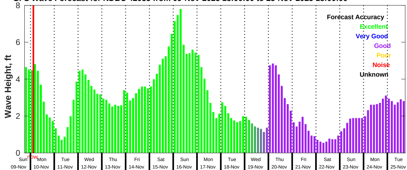
GFS Wave Forecast for NDBC 42035 from 09-Nov-2025 18:00:00 to 25-Nov-2025 18:00:00
