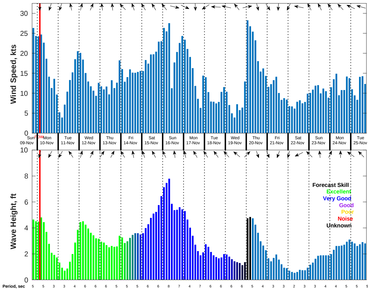
Wind & Wave Forecast for NDBC 42035 from 09-Nov-2025 18:00:00 to 25-Nov-2025 18:00:00
