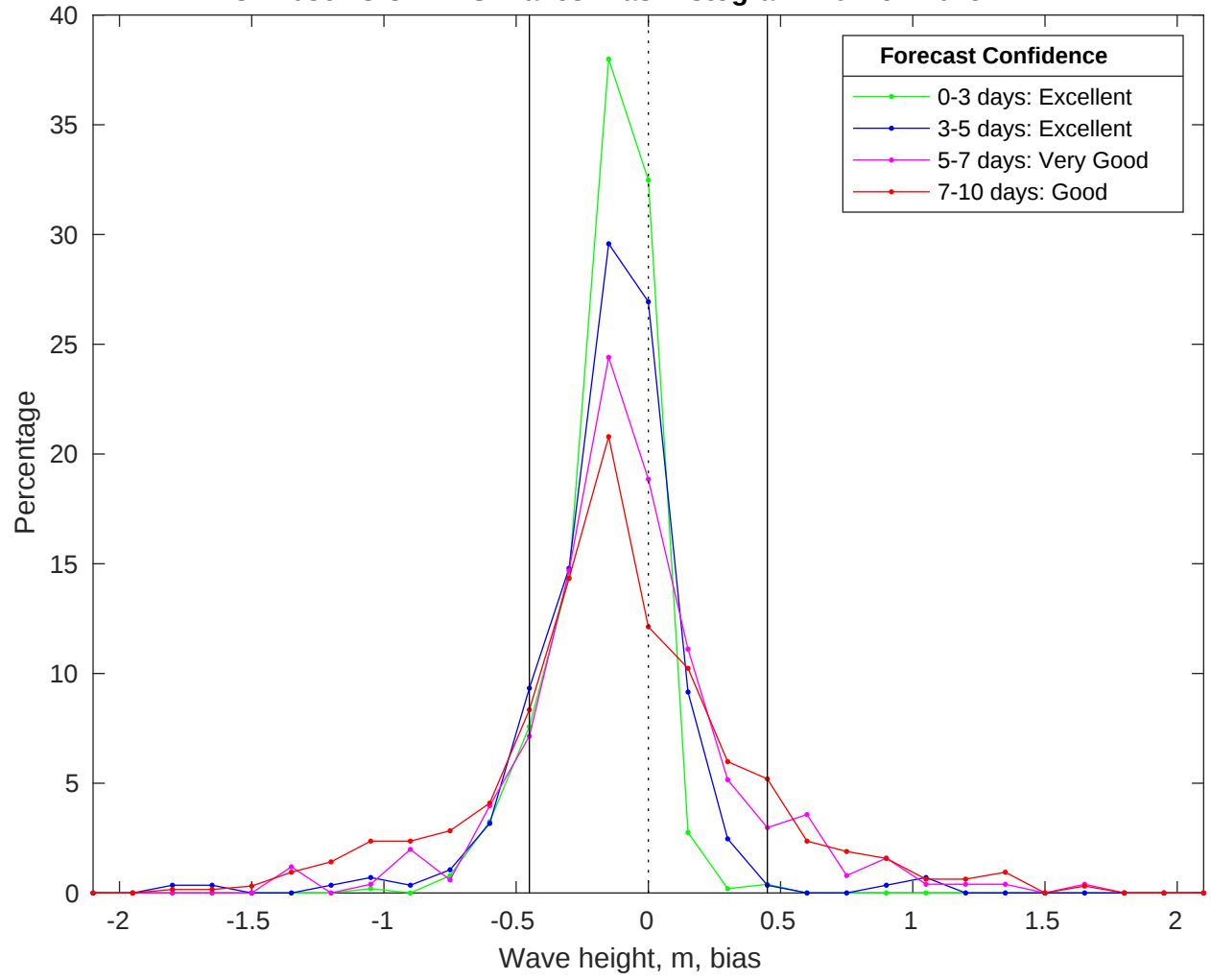
NDBC 42036 vs CMEMS Waves Bias Histogram: 10-Nov-2025
