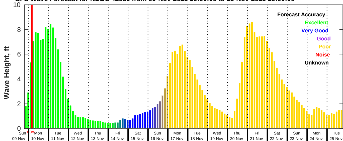
GFS Wave Forecast for NDBC 42036 from 09-Nov-2025 19:00:00 to 25-Nov-2025 19:00:00
