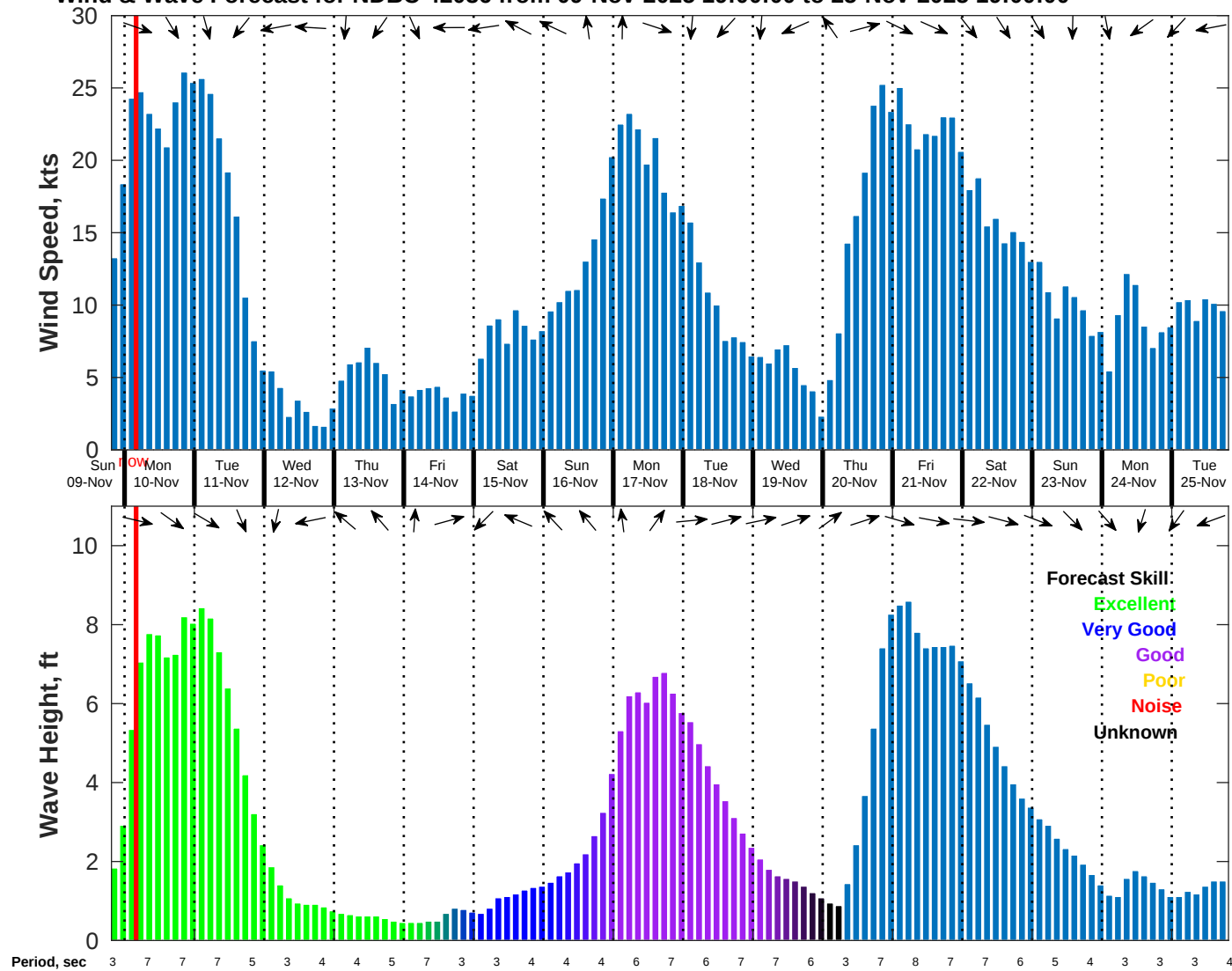
Wind & Wave Forecast for NDBC 42036 from 09-Nov-2025 19:00:00 to 25-Nov-2025 19:00:00
