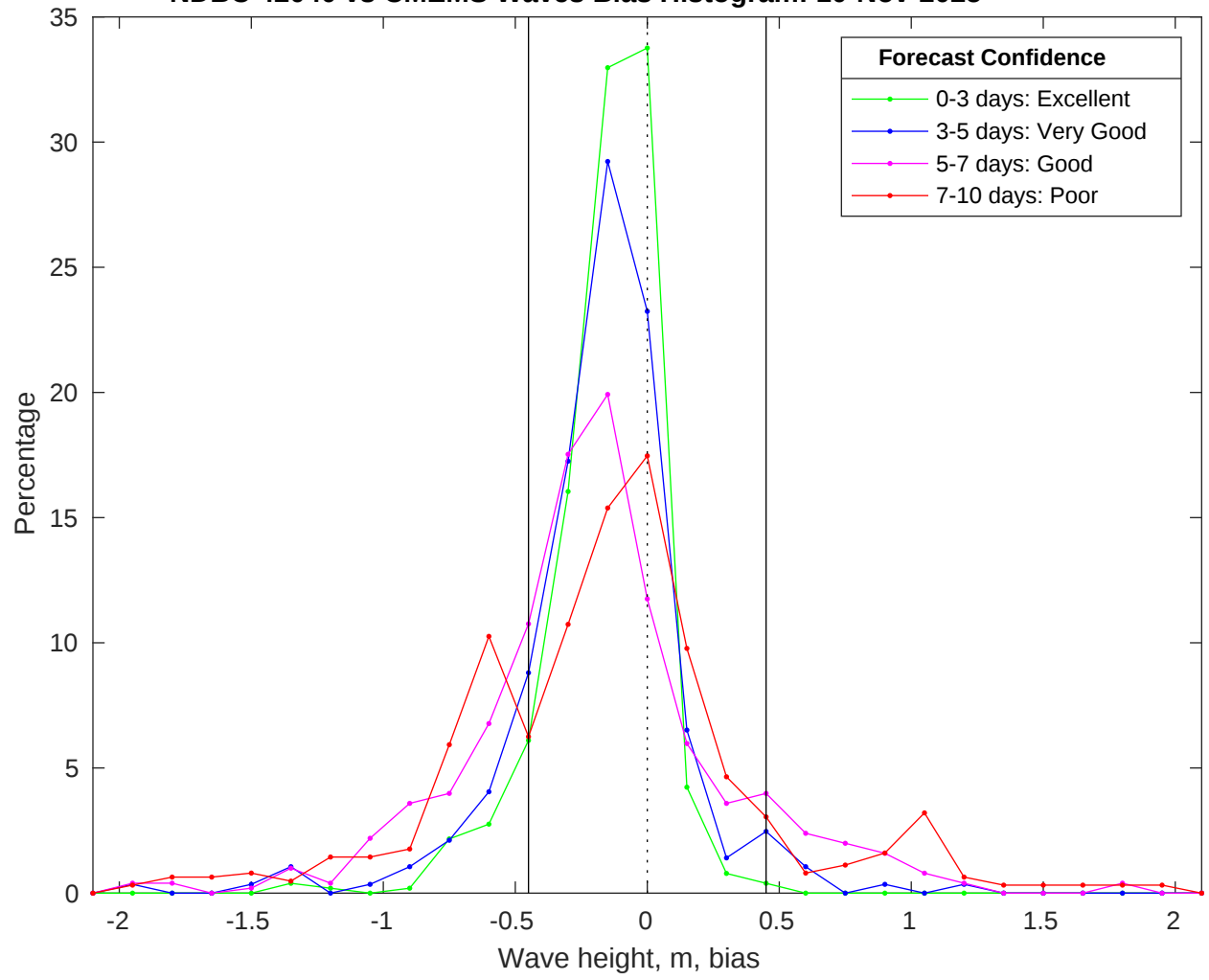
NDBC 42040 vs CMEMS Waves Bias Histogram: 10-Nov-2025
