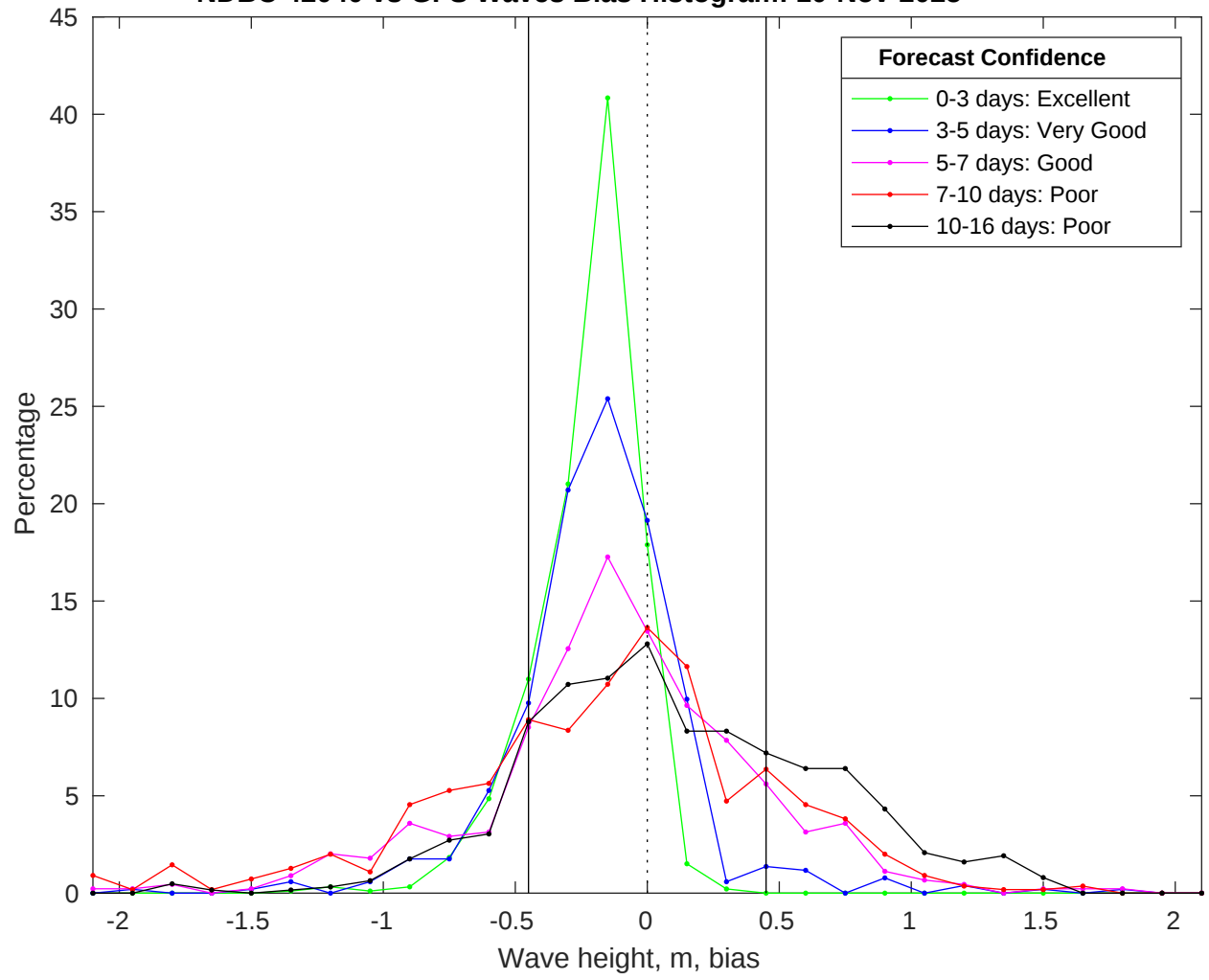
NDBC 42040 vs GFS Waves Bias Histogram: 10-Nov-2025
