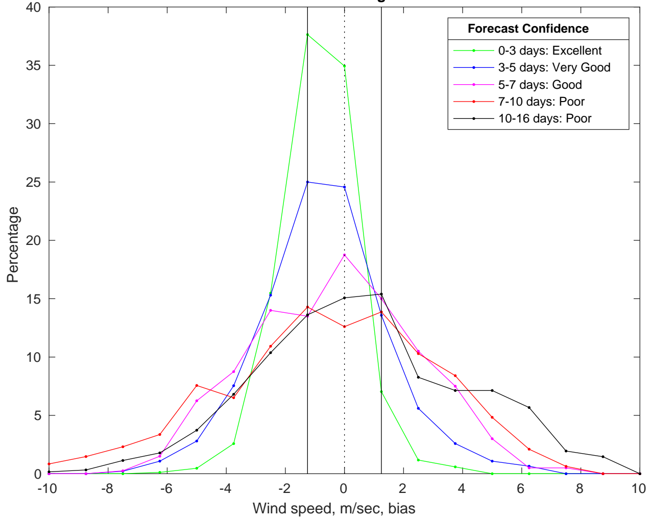
NDBC 42040 vs GFS Winds Bias Histogram: 10-Nov-2025
