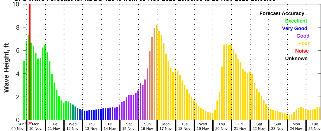
GFS Wave Forecast for NDBC 42040 from 09-Nov-2025 19:00:00 to 25-Nov-2025 19:00:00
