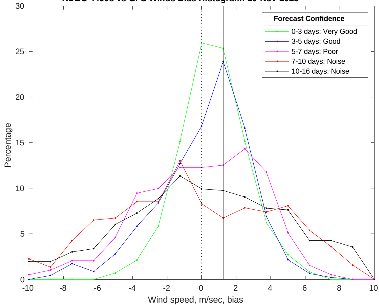
NDBC 44008 vs GFS Winds Bias Histogram: 10-Nov-2025
