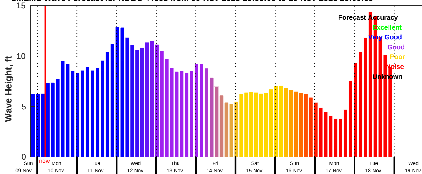
CMEMS Wave Forecast for NDBC 44008 from 09-Nov-2025 20:00:00 to 19-Nov-2025 20:00:00
