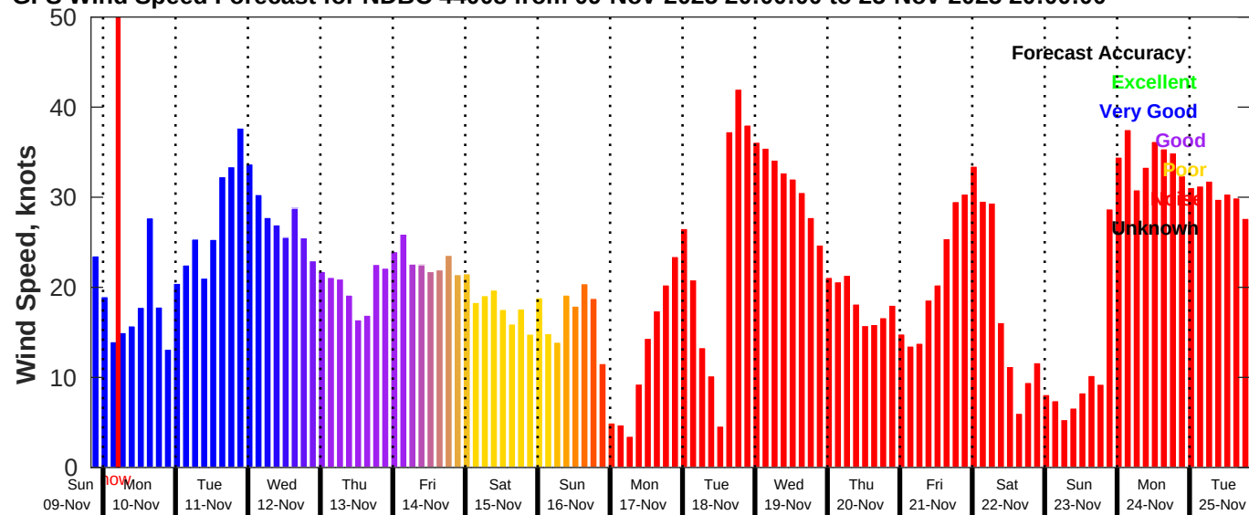
GFS Wind Speed Forecast for NDBC 44008 from 09-Nov-2025 20:00:00 to 25-Nov-2025 20:00:00
