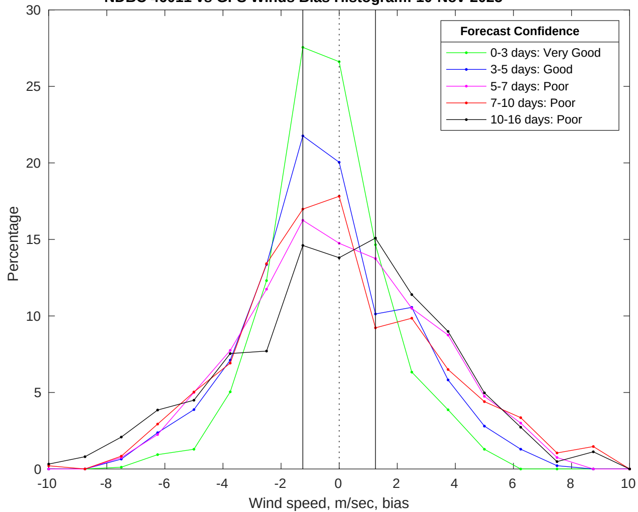
NDBC 46011 vs GFS Winds Bias Histogram: 10-Nov-2025
