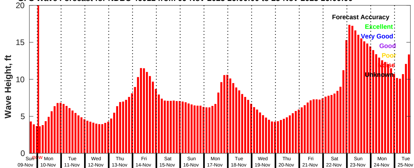
GFS Wave Forecast for NDBC 46011 from 09-Nov-2025 16:00:00 to 25-Nov-2025 16:00:00
