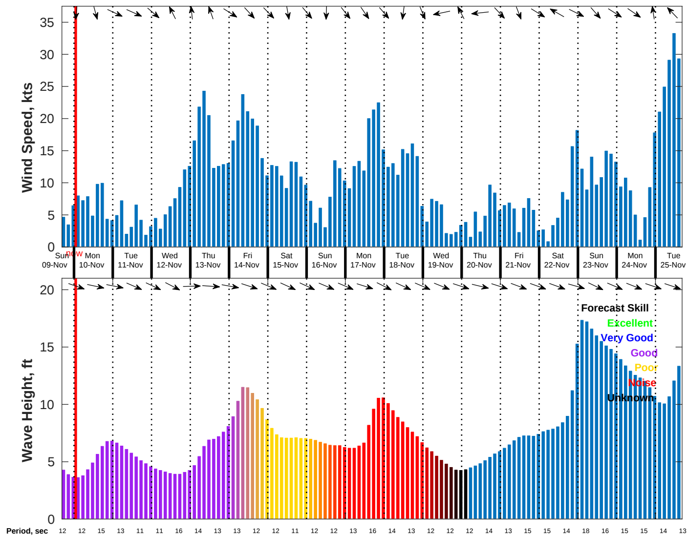
Wind & Wave Forecast for NDBC 46011 from 09-Nov-2025 16:00:00 to 25-Nov-2025 16:00:00
