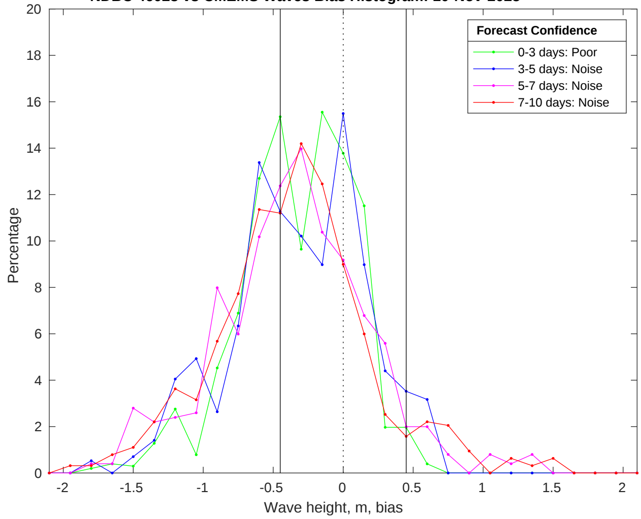
NDBC 46028 vs CMEMS Waves Bias Histogram: 10-Nov-2025
