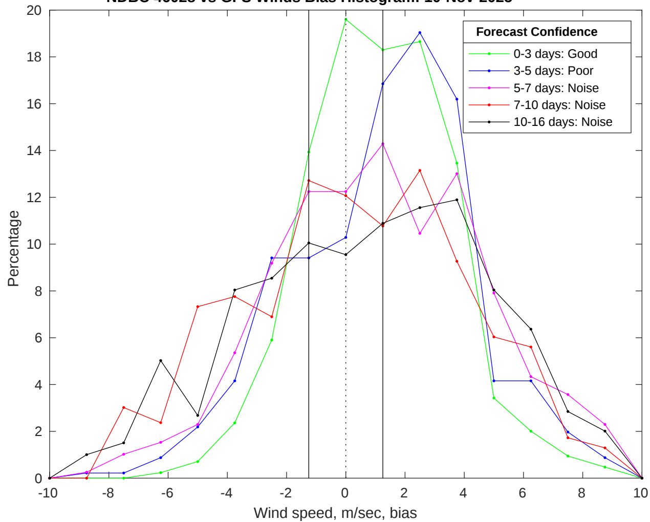
NDBC 46028 vs GFS Winds Bias Histogram: 10-Nov-2025
