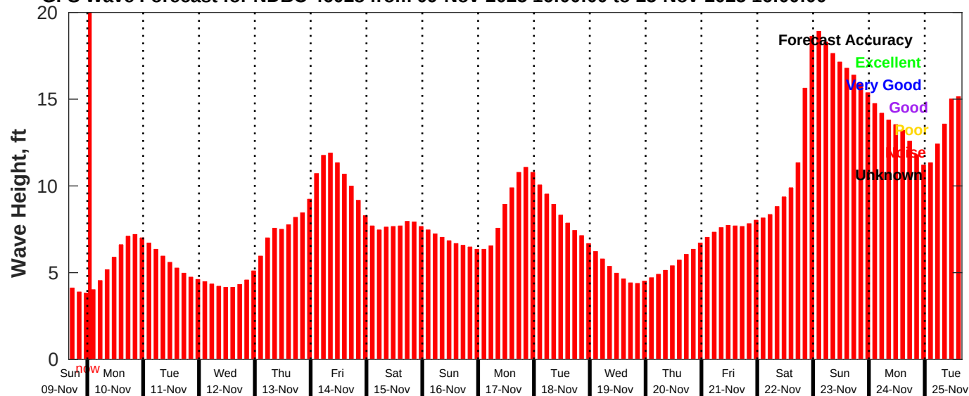
GFS Wave Forecast for NDBC 46028 from 09-Nov-2025 16:00:00 to 25-Nov-2025 16:00:00
