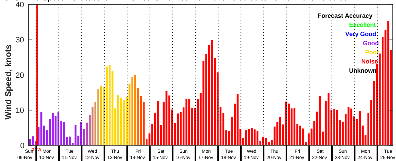
GFS Wind Speed Forecast for NDBC 46028 from 09-Nov-2025 16:00:00 to 25-Nov-2025 16:00:00
