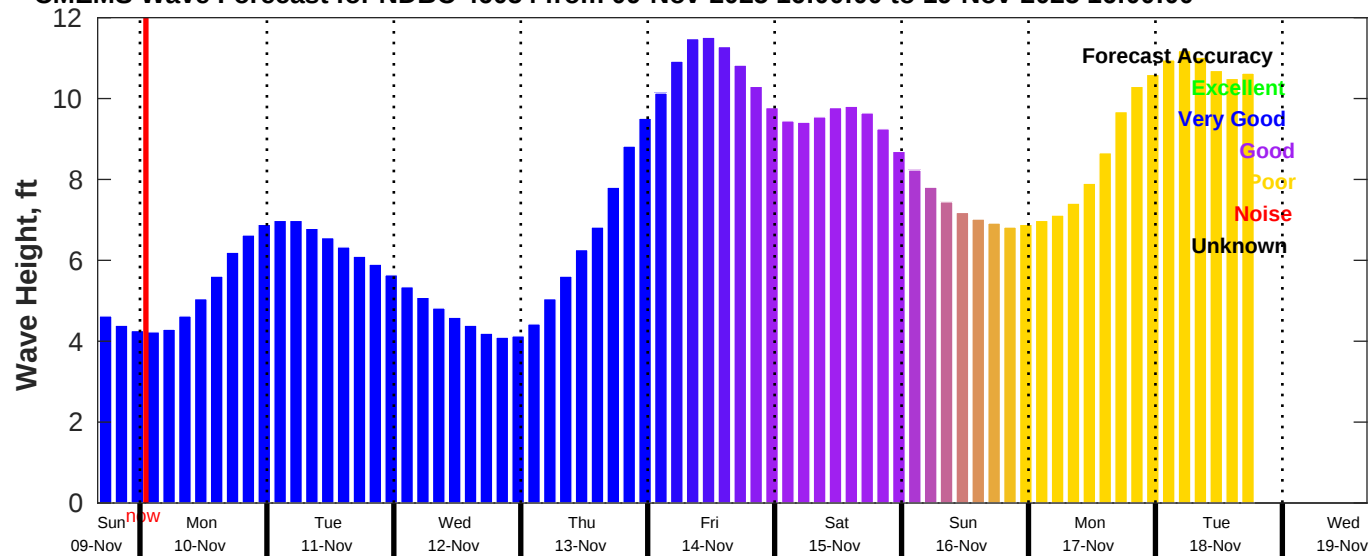
CMEMS Wave Forecast for NDBC 46054 from 09-Nov-2025 16:00:00 to 19-Nov-2025 16:00:00
