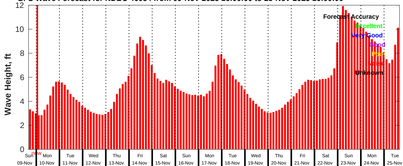
GFS Wave Forecast for NDBC 46054 from 09-Nov-2025 16:00:00 to 25-Nov-2025 16:00:00
