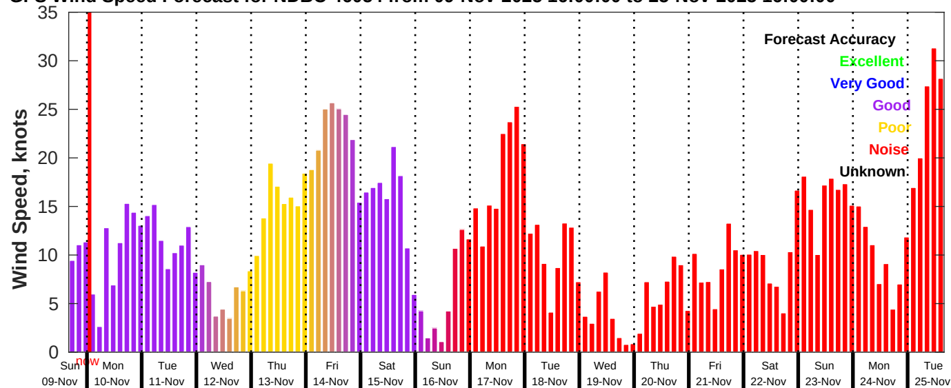
GFS Wind Speed Forecast for NDBC 46054 from 09-Nov-2025 16:00:00 to 25-Nov-2025 16:00:00
