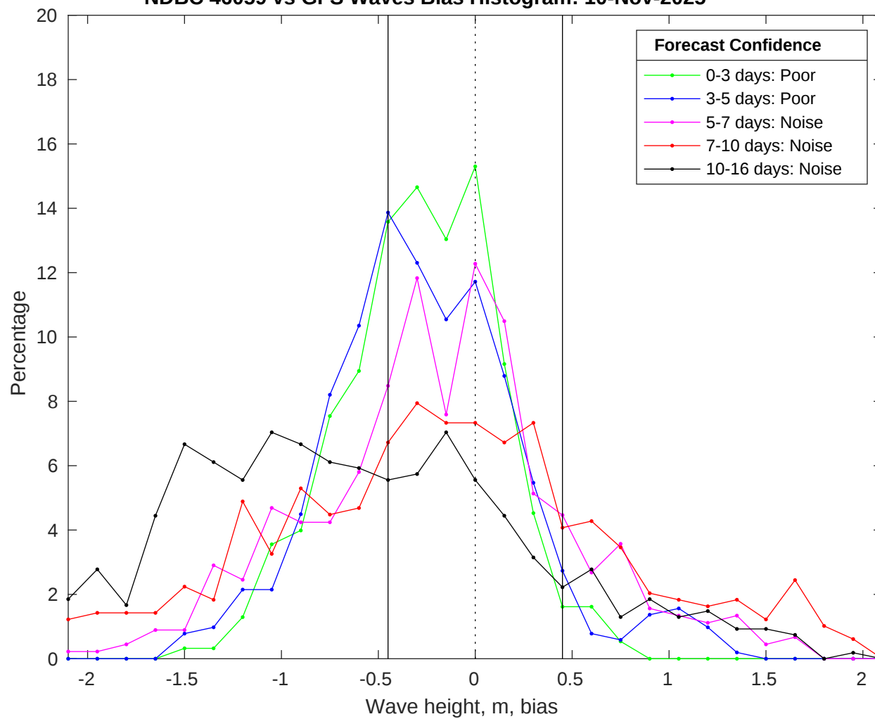
NDBC 46059 vs GFS Waves Bias Histogram: 10-Nov-2025
