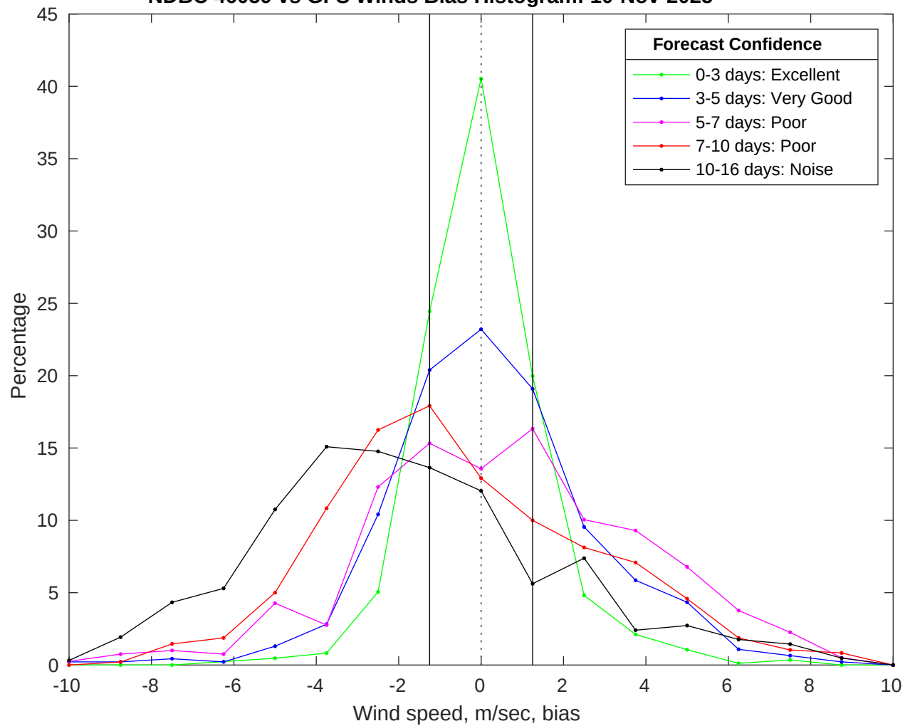
NDBC 46059 vs GFS Winds Bias Histogram: 10-Nov-2025
