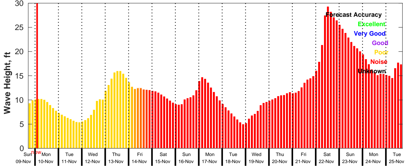
GFS Wave Forecast for NDBC 46059 from 09-Nov-2025 17:00:00 to 25-Nov-2025 17:00:00
