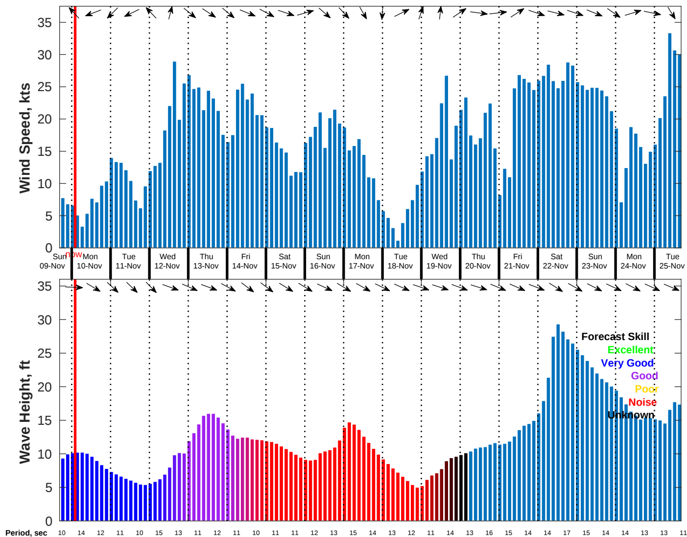
Wind & Wave Forecast for NDBC 46059 from 09-Nov-2025 17:00:00 to 25-Nov-2025 17:00:00
