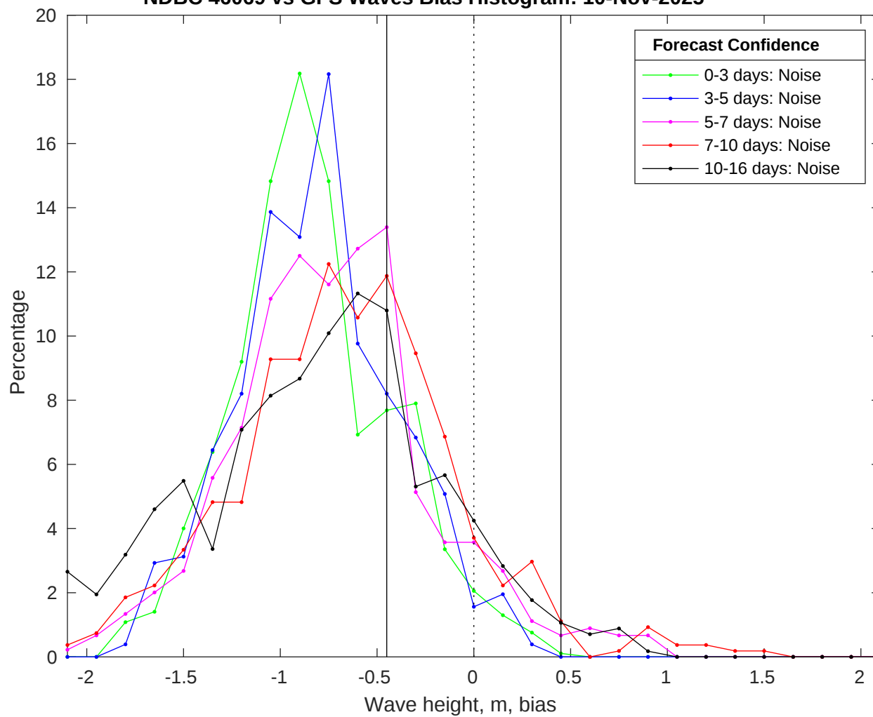
NDBC 46069 vs GFS Waves Bias Histogram: 10-Nov-2025
