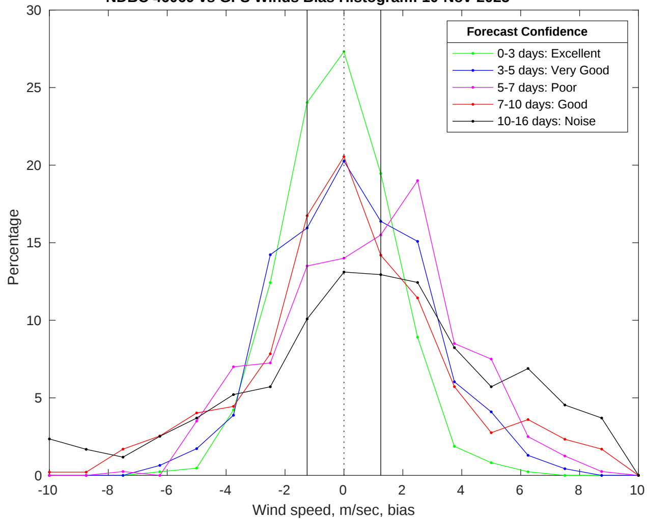
NDBC 46069 vs GFS Winds Bias Histogram: 10-Nov-2025
