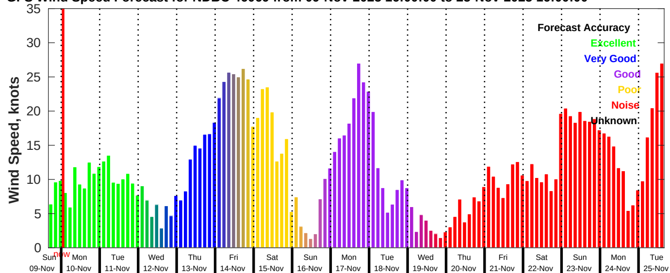
GFS Wind Speed Forecast for NDBC 46069 from 09-Nov-2025 16:00:00 to 25-Nov-2025 16:00:00
