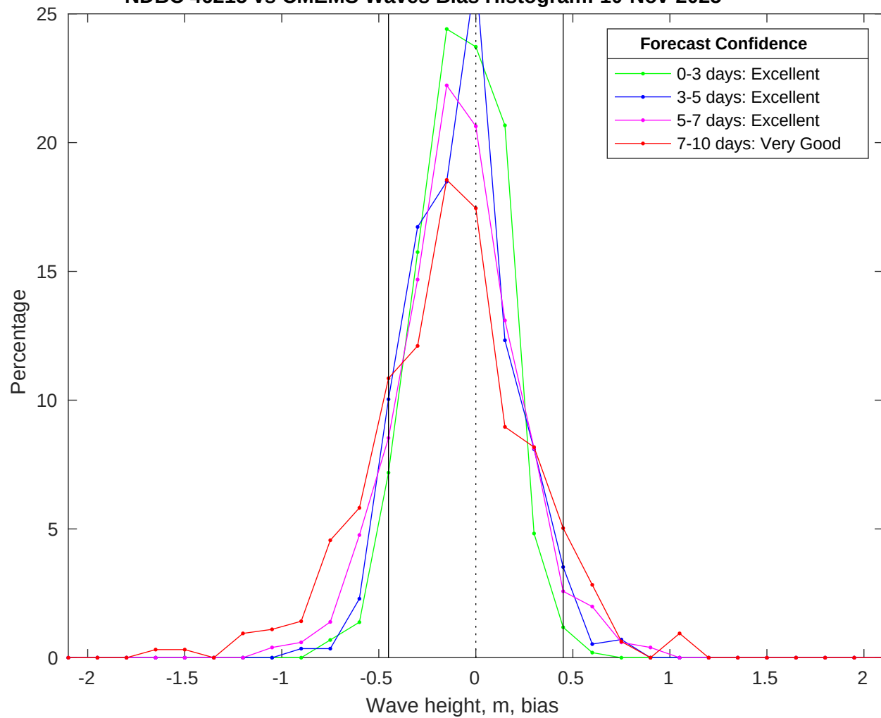
NDBC 46215 vs CMEMS Waves Bias Histogram: 10-Nov-2025
