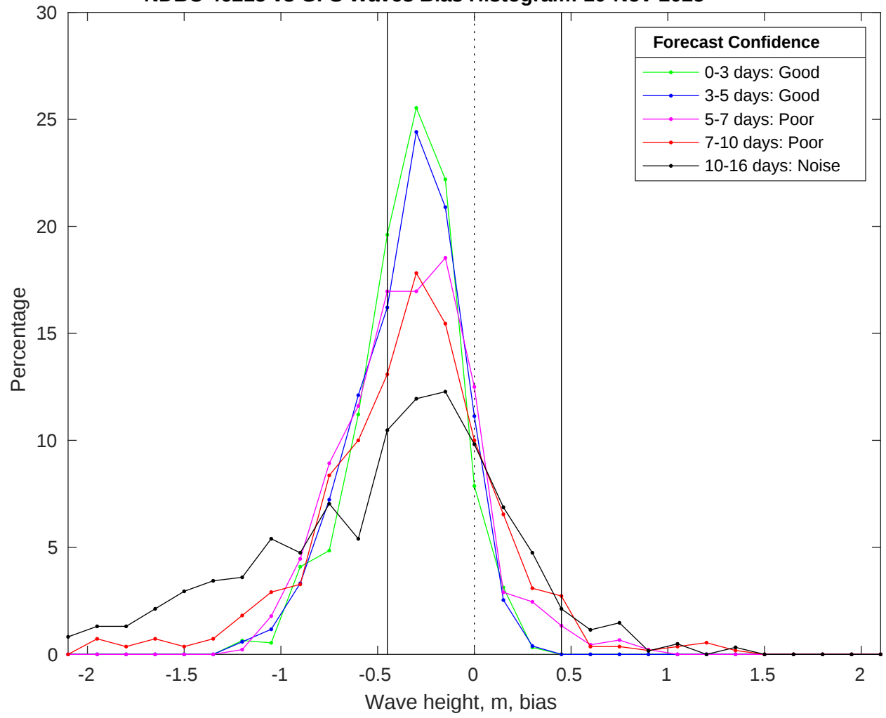
NDBC 46215 vs GFS Waves Bias Histogram: 10-Nov-2025
