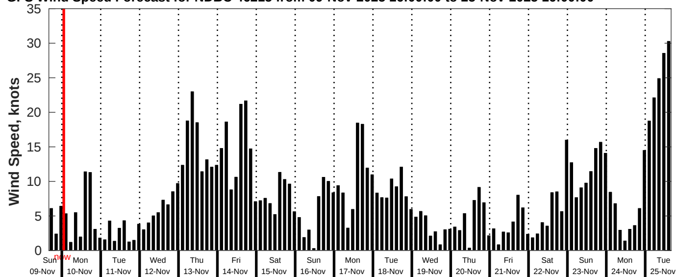
GFS Wind Speed Forecast for NDBC 46215 from 09-Nov-2025 16:00:00 to 25-Nov-2025 16:00:00
