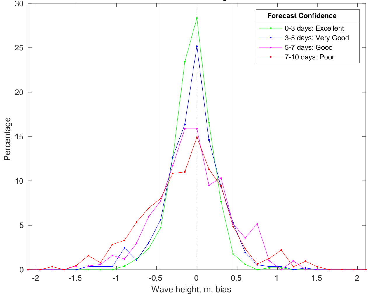
NDBC 46259 vs CMEMS Waves Bias Histogram: 10-Nov-2025
