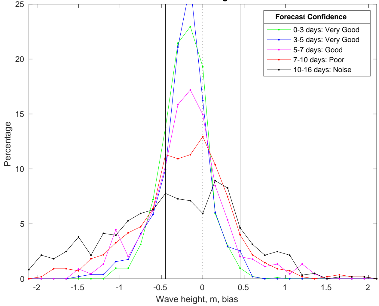
NDBC 46259 vs GFS Waves Bias Histogram: 10-Nov-2025
