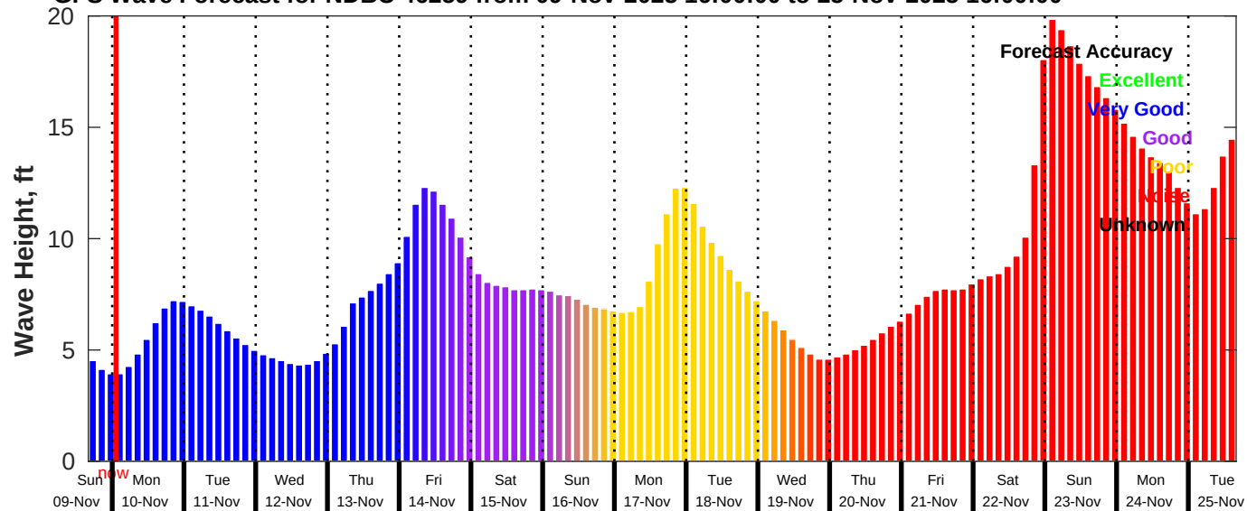
GFS Wave Forecast for NDBC 46259 from 09-Nov-2025 16:00:00 to 25-Nov-2025 16:00:00
